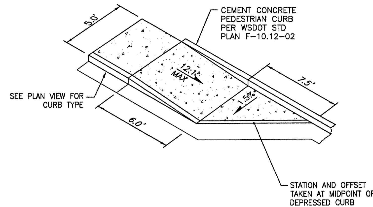
BICYCLE RAMP NOT TO SCALE
