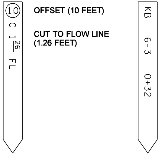
FRONT BACK STAKE FOR DRAINAGE
