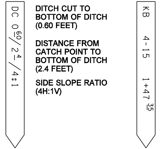
FRONT BACK STAKE FOR DITCH CONSTRUCTION
