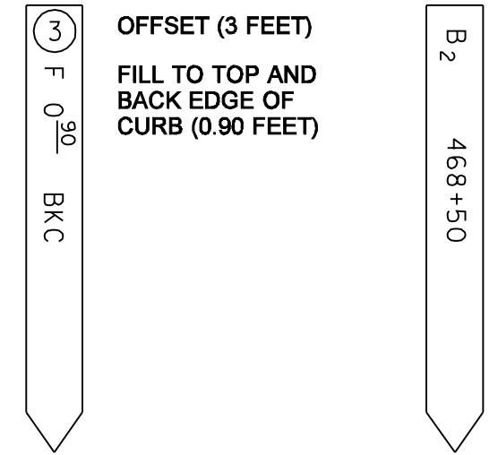
FRONT BACK STAKE FOR CURB/GUTTER
