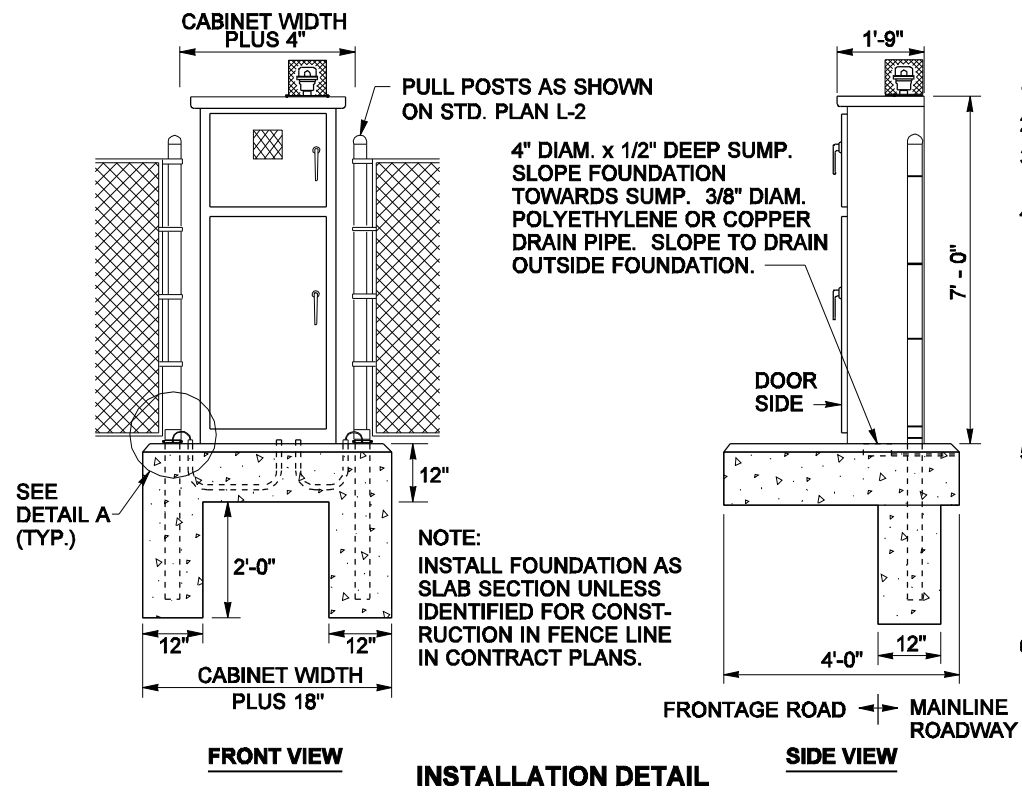
INSTALLATION DETAIL
