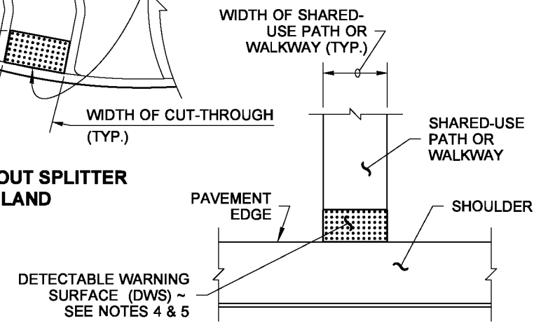
SHARED-USE PATH CONNECTION
