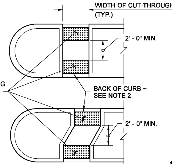
MEDIAN CUT-THROUGH
