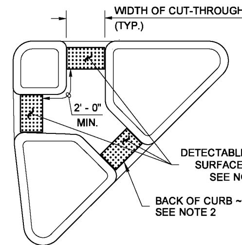
ISLAND CUT-THROUGH
