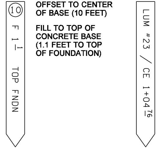
FRONT BACK STAKE FOR FOUNDATION OF LUMINAIRES, SIGNALS OR SIGN STRUCTURES
