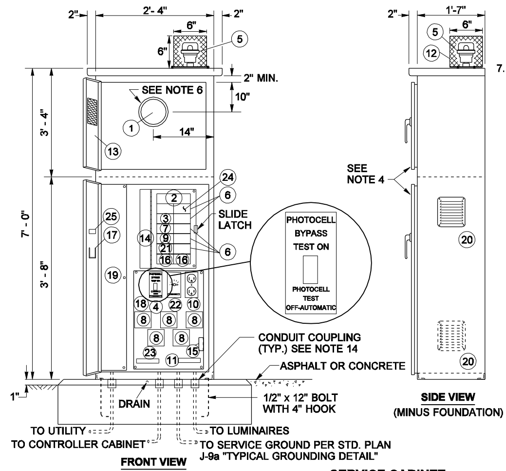
SERVICE CABINET
