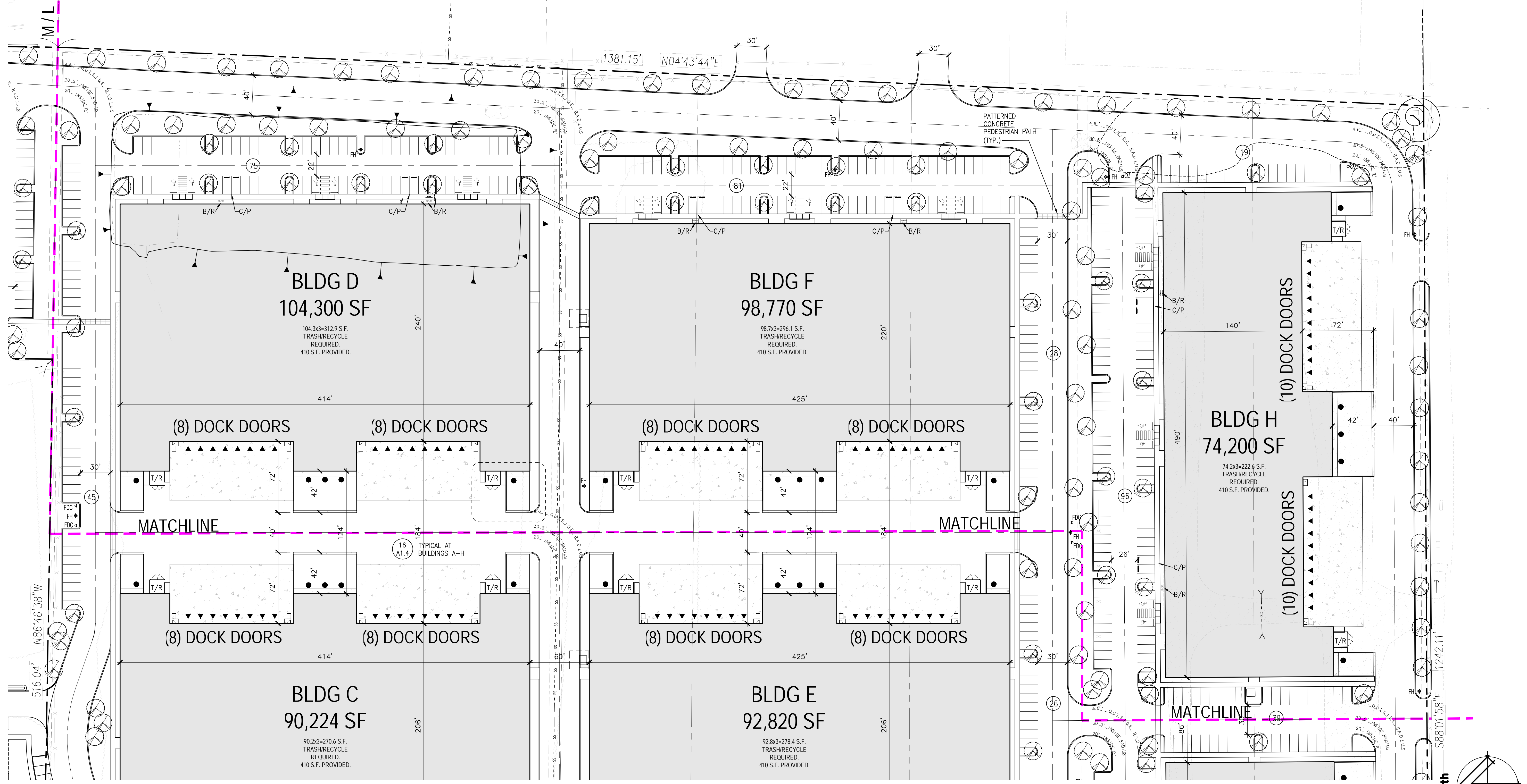
11 PARTIAL SITE PLAN - SOUTHEAST END Scale: 1"=50'-0"
